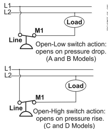
Figure 5: Typical Wiring for SPST Open-Low Switch and Open-High Switch (P70A, B, C, D and P170A, C, D Type Models)
