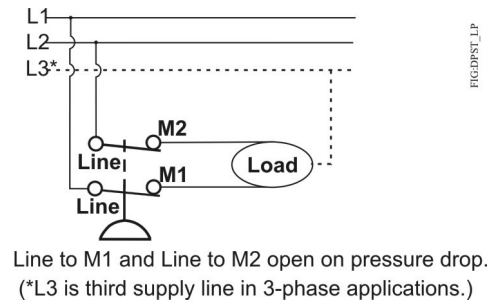
Figure 8: Typical Wiring for DPST Switch (P72A and B Type Models)
